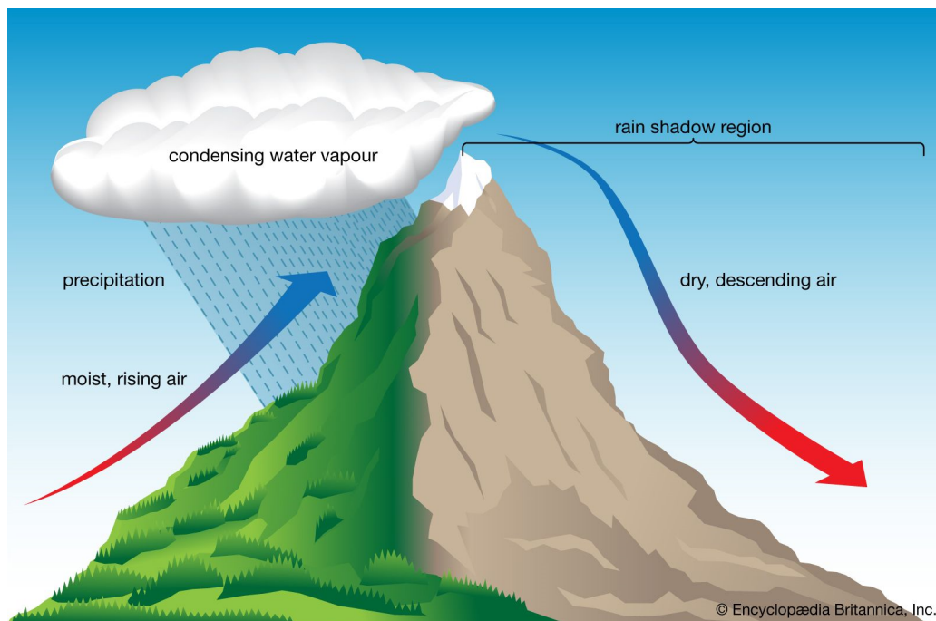
Figure 6-8: Orographic precipitation 16
