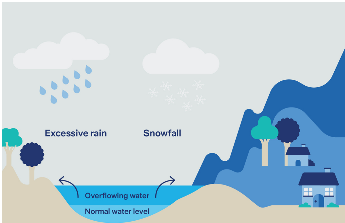
Figure 6-2: Riverine Flooding 3
